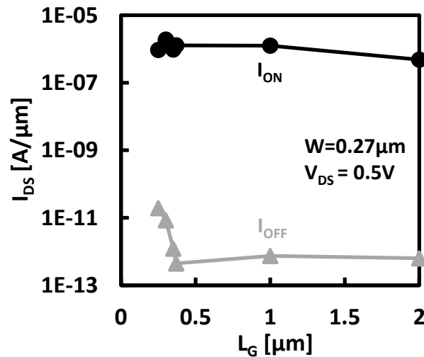
Fig. 3.7 Measured TFET I_{ON} and I_{OFF} vs. L_G . I_{OFF} corresponds to the minimum I_{DS} ; I_{ON} corresponds to I_{DS} for 0.5 \text{V} gate voltage swing.
