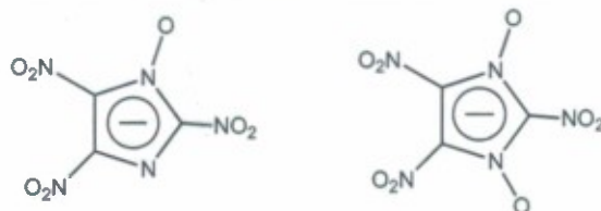
Figure 8. 2,4,5-trinitroimidazole oxide and dioxide targets.
