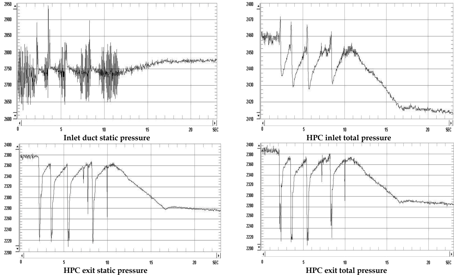
Figure 22: Surge inception in the time domain acquired with the conventional pressure probes, obtained by throttling of the HPC with Core blockage mechanism, for NHPC = 87% and 240° inlet flow distortion.
