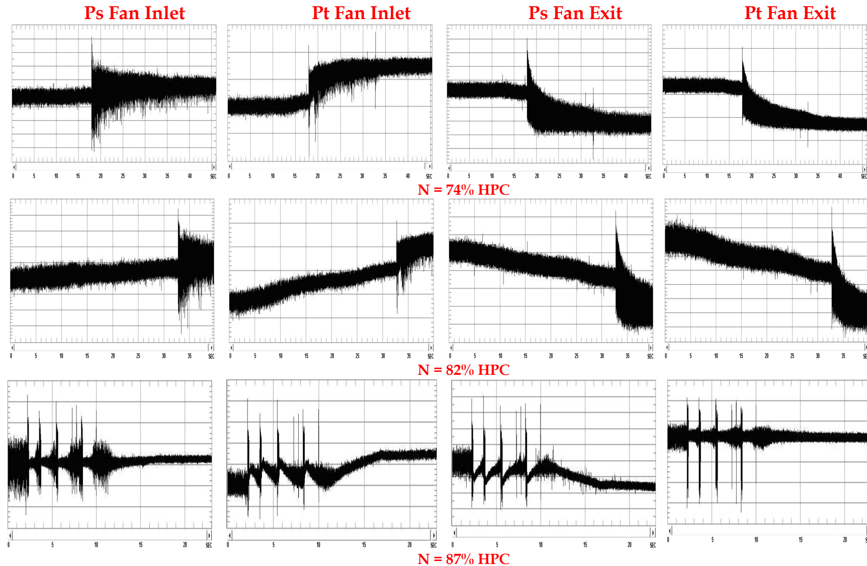
Figure 20: Stall inception in the time domain as acquired with the Kulite, for different rotational speeds of the HPC, obtained by throttling the HPC with the Core blockage mechanism, and with 240^\circ inlet flow distortion
