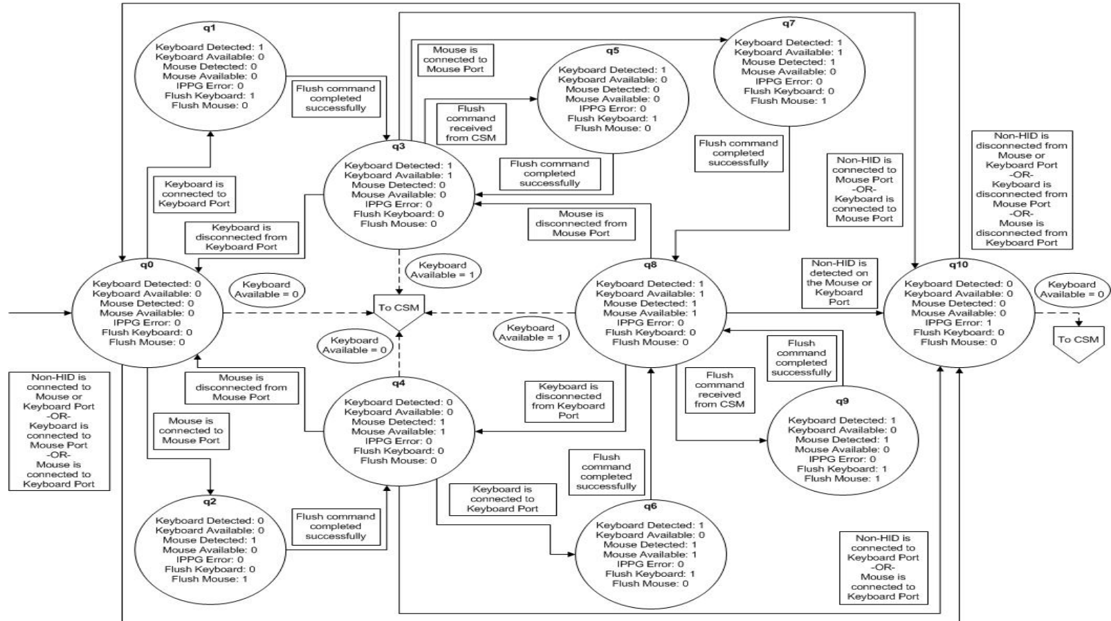
Figure 22. IPPG State Machine Including Flush Command States
