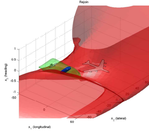
(b) Capture (light, green) and collision (dark, red) sets for Rejoin.
