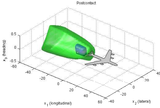
(a) Postcontact capture set (light, green) and Stationary 3 invariant set (dark, blue).
