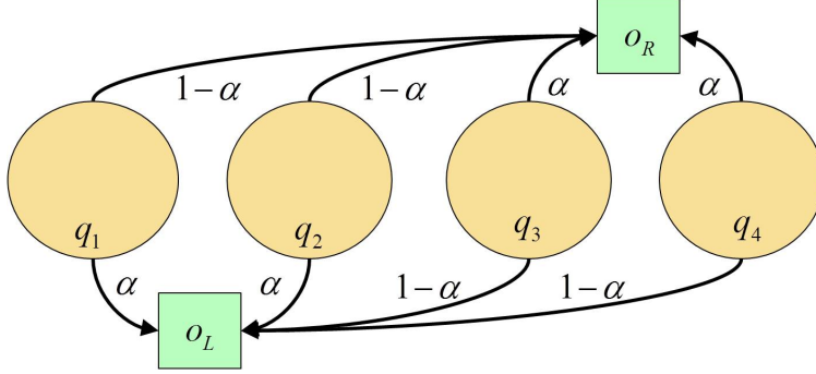
Figure 5.4: State observation diagram for POMDP example.
