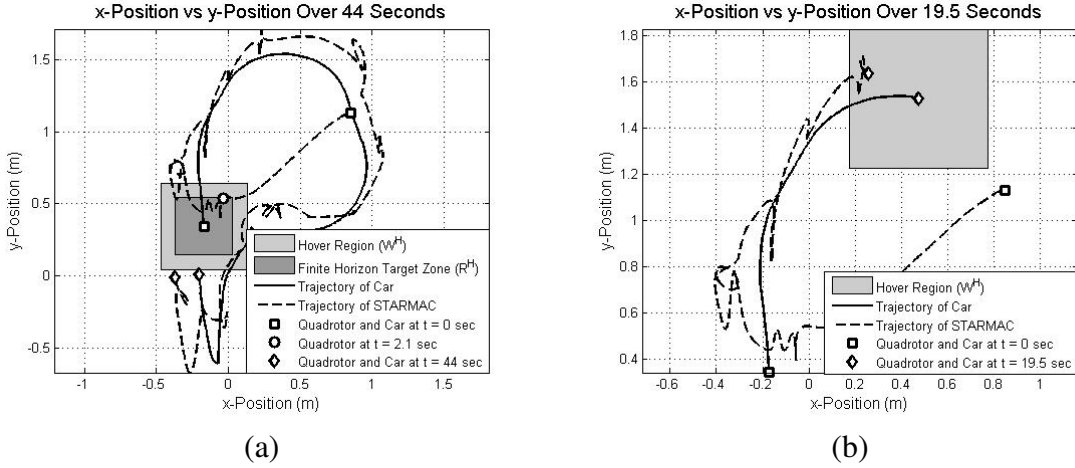
Figure 3.9: Results from car following experiment: (a) x-Position (m) and y-Position (m) trajectories of STARMAC and ground vehicle over 44 second; (b) Snapshot of trajectories at t = 19.5 .
