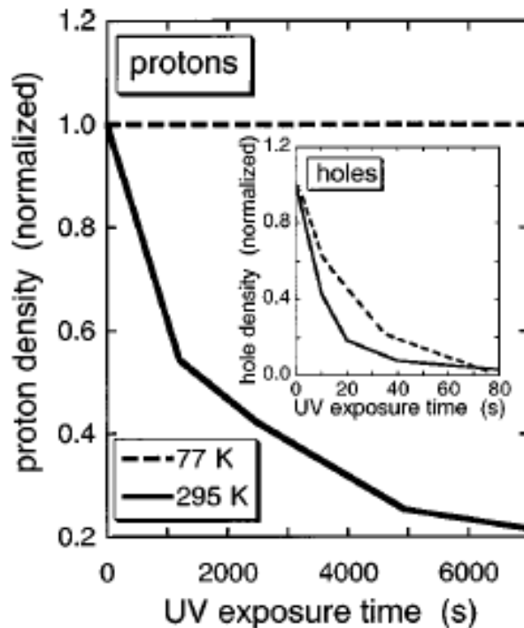
Fig. 6. Relative charge neutralization rates for trapped holes and protons in \sim 1 \mu m oxides grown on zone-melt recrystallized SiO 2 during 5 eV ultraviolet illumination for the same exposure conditions at 295 K and 77 K. This energy is high enough to inject electrons over the 3.1 eV Si-to-SiO 2 barrier, but too low to create electron-hole pairs in SiO 2 . (After K. Vanheusden, et al. Appl. Phys. Lett. , 72, no. 1, pp. 28-30, 1998.)
