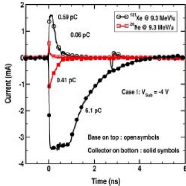
Fig. 108. JYFL -- ion LET comparison for Case 1. Neon and xenon transients captured at JYFL demonstrating device response to two extreme LETs, 3.7 MeV \text{cm}^2/\text{mg} for the neon ions and 60 MeV \text{cm}^2/\text{mg} for the xenon ions; the integrated charge is labeled next to each curve.
