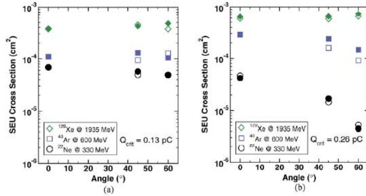
Fig 97. Plots (a) and (b) show the calibrated results of the computer simulations for the entire 127-stage shift register. In each case the open symbols are the data from Fig. 95 and the closed symbols are the derived simulation results. (a) Baseline design heavy ion calibration; (b) RHBD heavy ion calibration.
