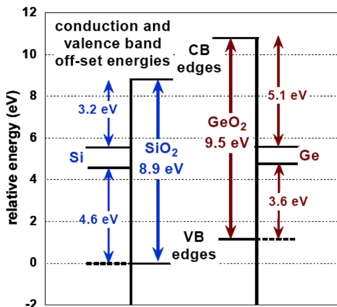
Fig. 48. c-Si and c-Ge band edge alignments with SiO 2 and GeO 2 , respectively.
