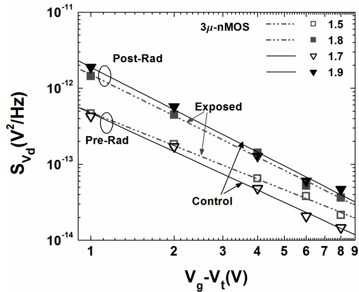
Fig. 3. SVD at \sim 10 Hz as a function of V_g - V_t for 3\ \mu\text{m} \times 16\ \mu\text{m} nMOS transistors from the control and moisture-exposed parts, before and after 500 krad(SiO 2 ) total dose irradiation.
