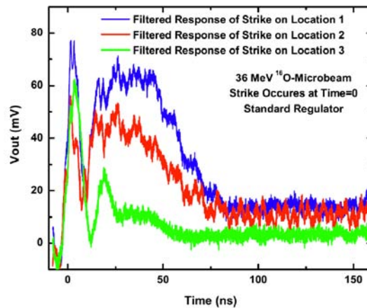
Fig. 16. Single-event transient response of the regulator for three different strike locations.
