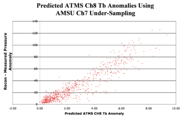
Figure 7. Predicted ATMS channel 8 Tb anomalies created using AMSU channel 7 adjusted to the ATMS scan resolution.
