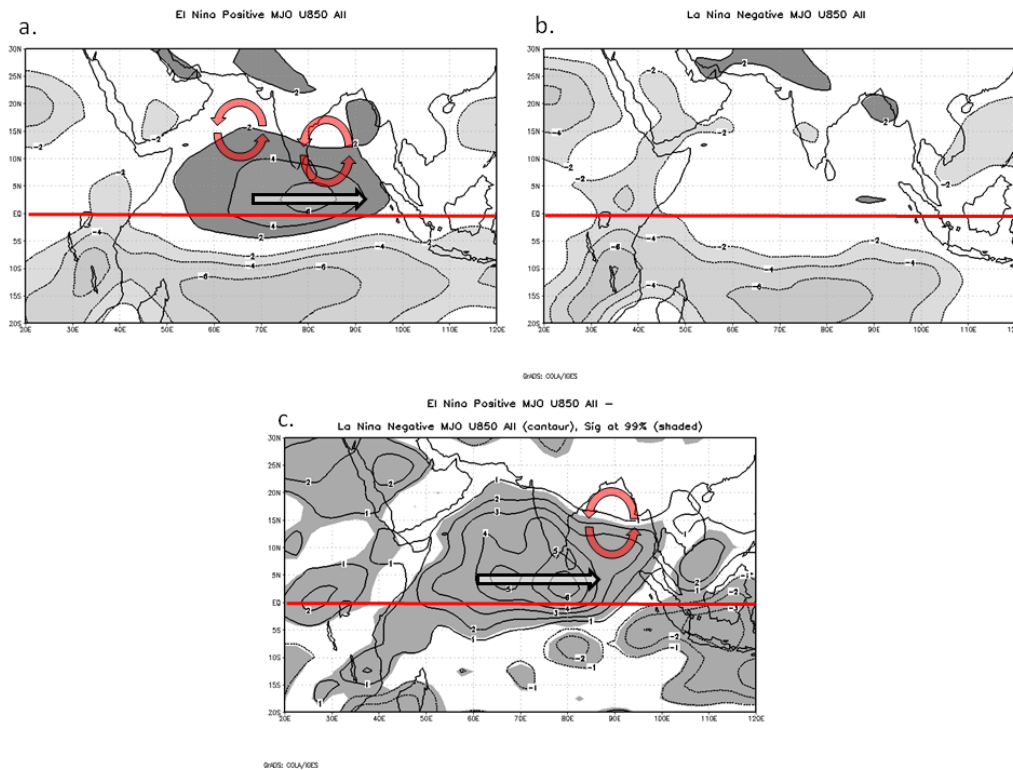
Figure 22. Composite U850 winds ( \text{m s}^{-1} ) when the ENSO and MJO are: (a) El Niño and positive MJO, (b) La Niña and negative MJO, and (c) El Niño/positive MJO - La Niña/negative. Shaded areas define 99% statistical significance.
