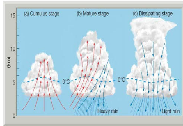
Figure 1. Single-cell or Airmass Thunderstorm characterized by the individual cell that is comprised of three short phases: (a) cumulus, (b) mature, and (c) dissipating. (Image from http://weatherblog.nbcactionnews.com/its-mothers-day-any-t-storms-coming-our-way/ )
