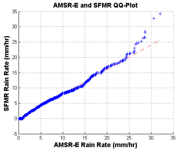
Figure 32. Statistical characteristics of the SFMR and AMSR-E rain rates for combined inner-core cases defined as (a) rain rate frequencies, (b) cumulative distribution functions, and (c) quantile-quantile plots.
