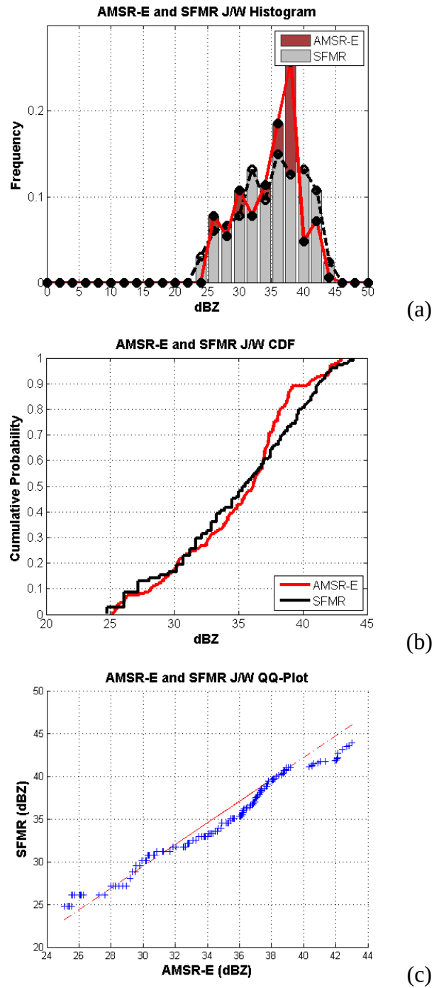
Figure 35. Statistical characteristics of the SFMR and AMSR-E J/W dBZ for TY Sinlaku on 12 Sep defined as (a) rain rate frequencies, (b) cumulative distribution functions, and (c) quantile-quantile plots.
