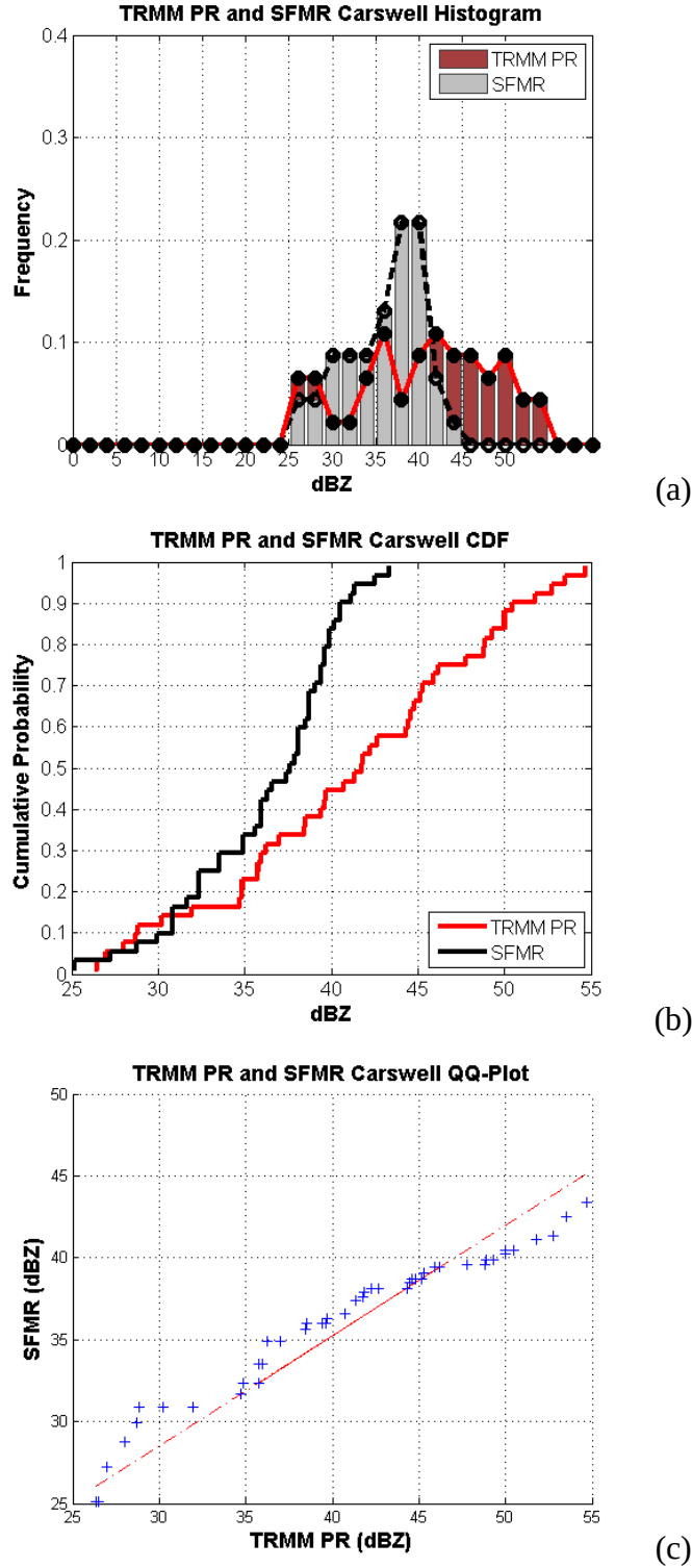
Figure 39. Statistical characteristics of the SFMR and TRMM PR Carswell dBZ for TY Sinlaku on 12 Sep defined as (a) rain rate frequencies, (b) cumulative distribution functions, and (c) quantile-quantile plots.
