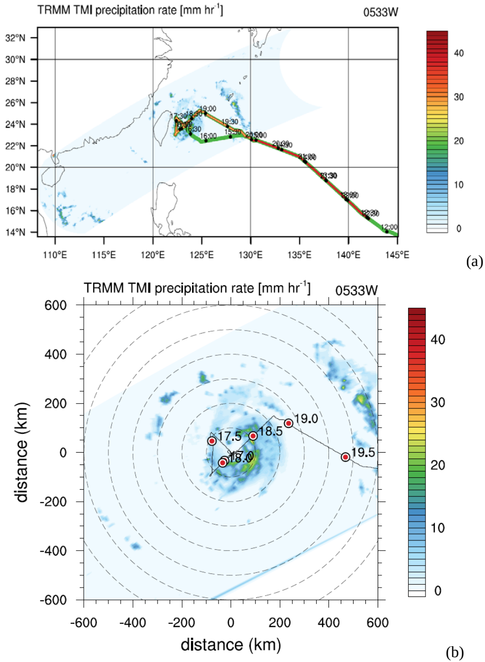
Figure 20. As in Figures 10 and 11, except for the TRMM TMI and (a) Earth-relative flight track and (b) storm-relative flight track for TY Sinlaku on 12 Sep 2008.
