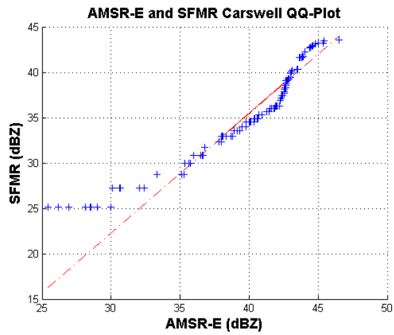
Figure 49. Carswell Statistical characteristics of the SFMR and AMSAR-E Carswell dBZ for TY Jangmi on 27 Sep defined as (a) rain rate frequencies, (b) cumulative distribution functions, and (c) quantile-quantile plots.
