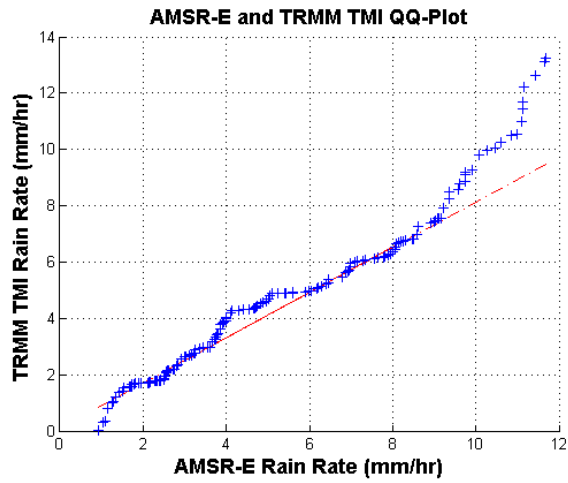
Figure 23. Statistical characteristics of the AMSR-E and TRMM TMI rain rates for TY Sinlaku on 12 Sep defined as (a) rain rate frequencies, (b) cumulative distribution functions, and (c) quantile-quantile plots.
