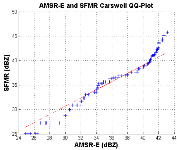
Figure 52. Statistical characteristics of the SFMR and AMSR-E Carswell dBZ for TY Fanapi on 17 Sep defined as (a) rain rate frequencies, (b) cumulative distribution functions, and (c) quantile-quantile plots.
