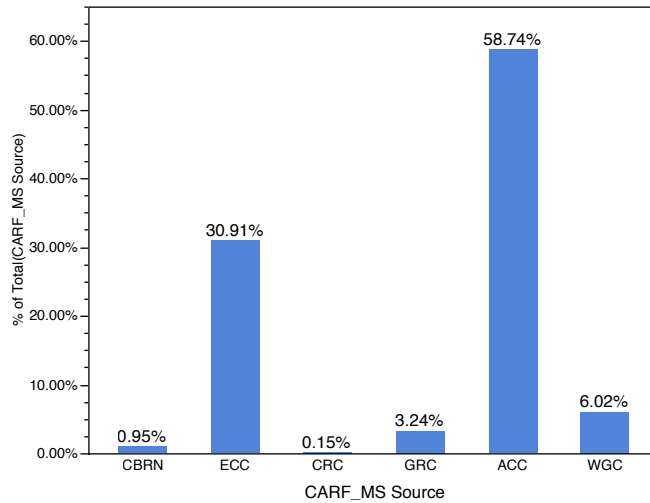
Figure 2-4. Obtained MS CARFs by Source.
