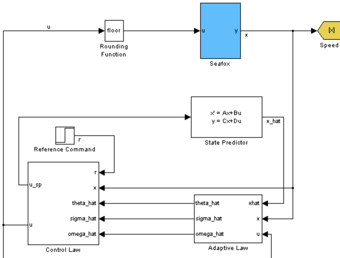
Figure 20. L_1 Adaptive Controller
