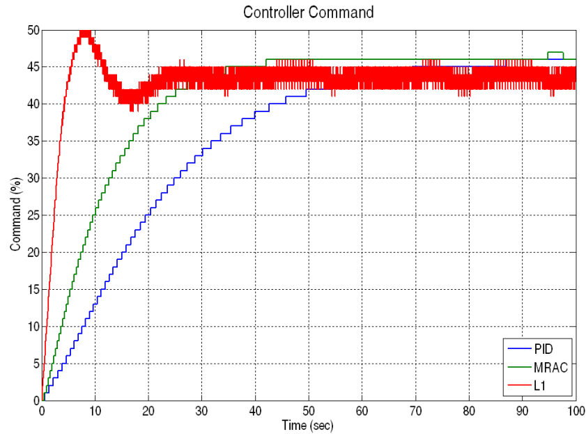
Figure 24. Controller Response: 3 m/s Reference Command, No Disturbance
