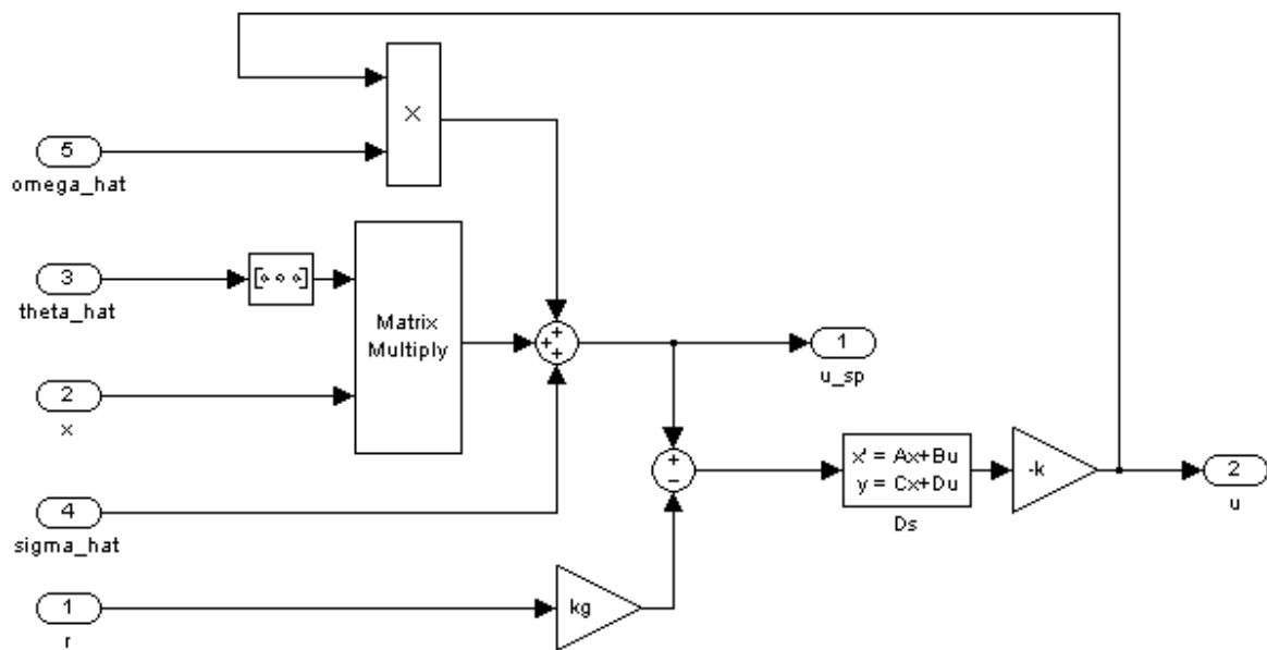
Figure 21. L_1 Control Law
