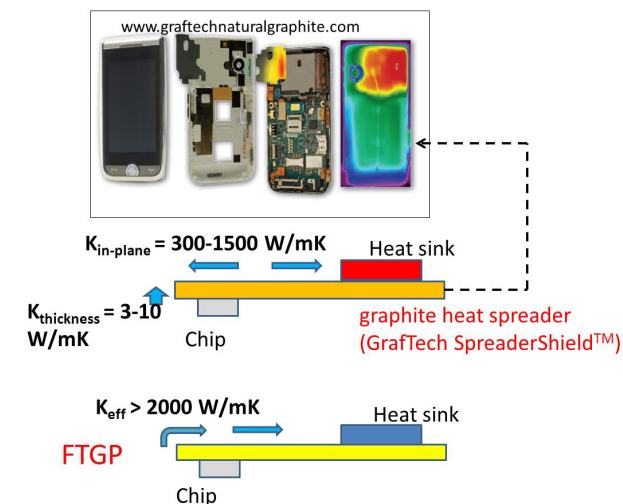
Figure 2. Illustration of a graphite heat spreader application, and FTGP's enhanced capability to replace graphite.
