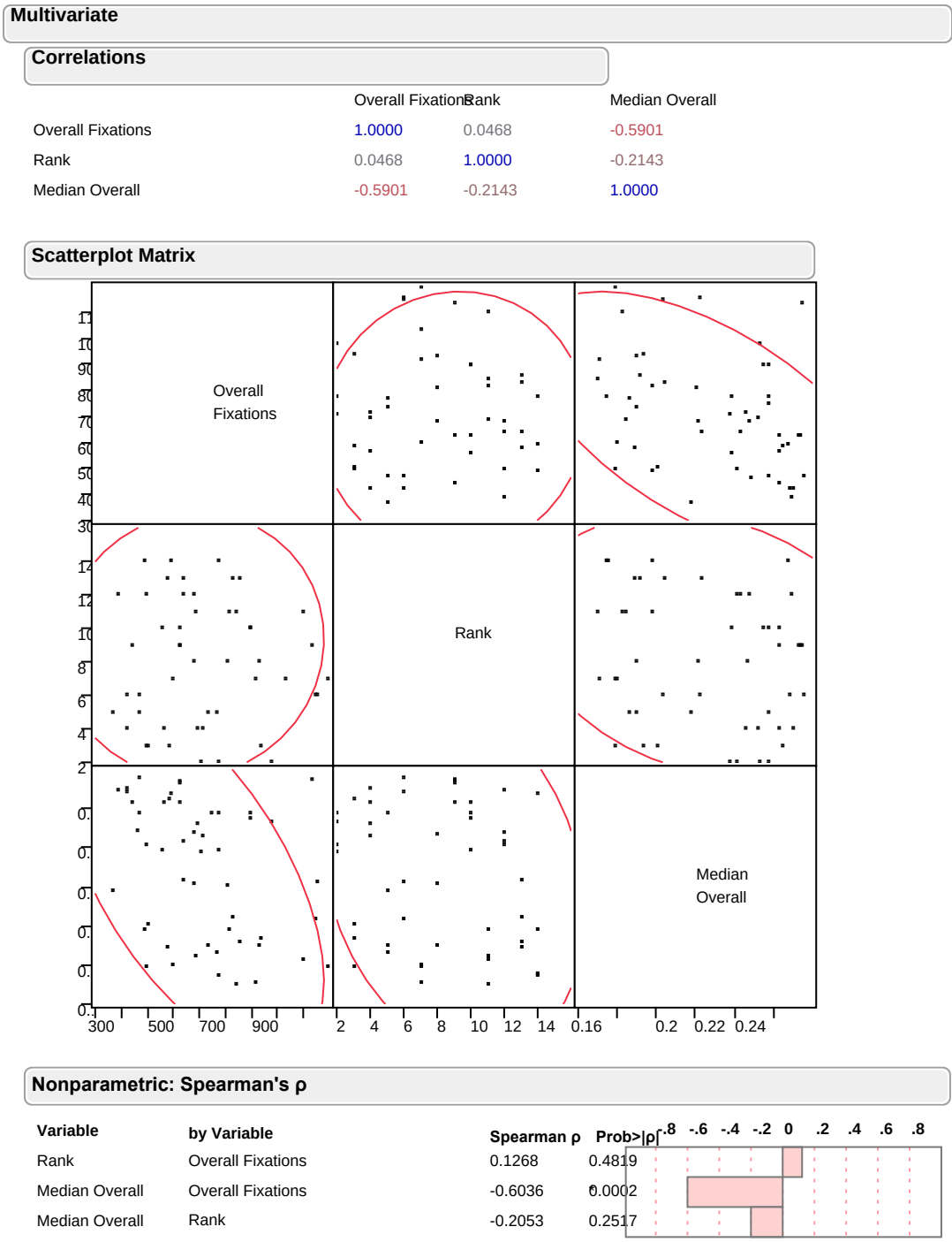
Figure 13. Multivariate Overall Median Dwell Times, Overall Mean Fixations, Ranked Experience
