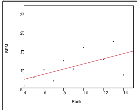
Bivariate Fit of BPM By Rank Scen=3
