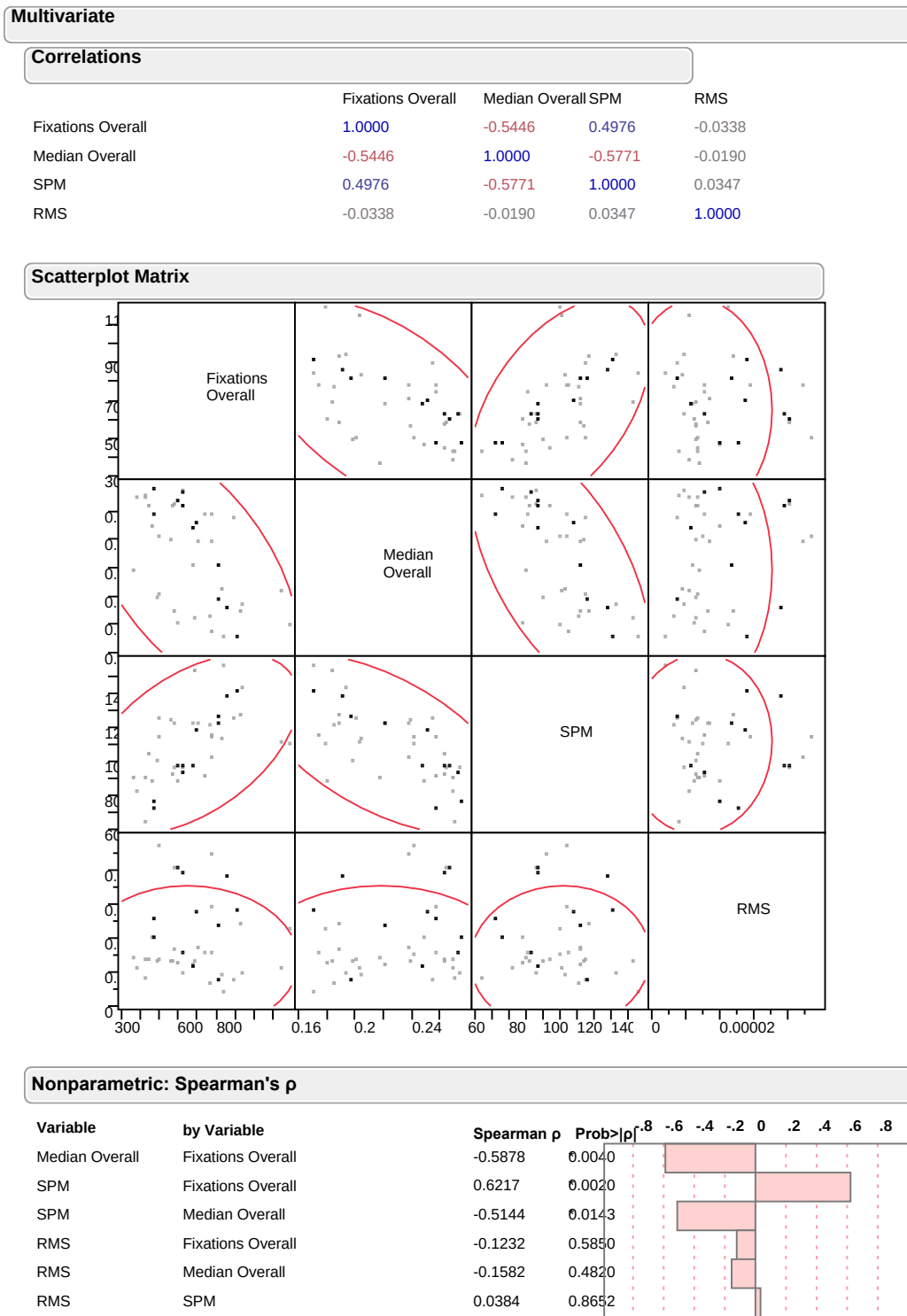
Figure 18. Multivariate Navigation RMS Error, Median Dwell, Fixation Count, Saccades per Minute
