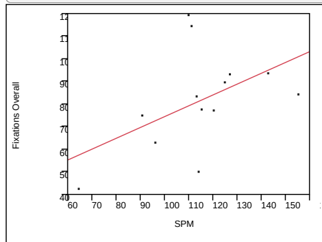
Bivariate Fit of Fixations Overall By SPM Scen=2
