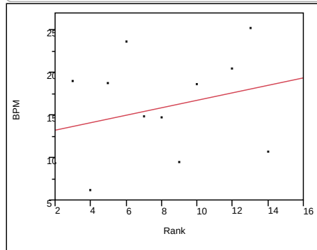
Bivariate Fit of BPM By Rank Scen=2
