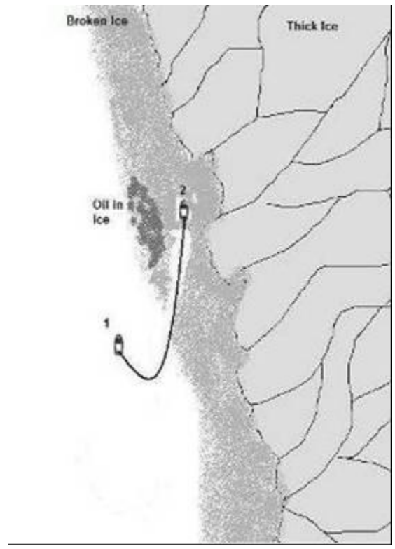
Figure 24. Maneuvering behind oil-saturated rubble ice.
