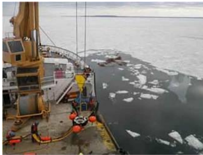
Figure 9. Helix skimmer being prepared for deployment in open water pocket surrounded by extensive ice sheet.
