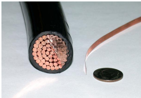
Figure 1. Commercially available 400A-class wires of Cu (left) and \text{YBa}_2\text{Cu}_3\text{O}_{7-z} (YBCO) middle (at 77K operation temperature), compared in size to a dime. Interestingly, the superconducting volume of the YBCO wire which is \sim 0.4\text{cm} \times 0.01\text{cm} is \sim 1\% of the volume shown, with the balance being \sim 0.005 cm thick metal-alloy substrate and \sim 0.005 cm thick copper layer for stabilization in case of quench. The volume and weight of this Cu wire compared to YBCO is \sim 800:1 , and the ratio for comparing multiple 2/0 Cu wires with 400 A capacity to YBCO is \sim 400:1 .
