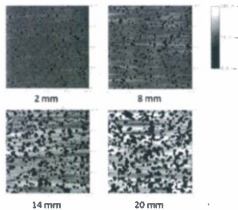
Fig. 6.3. AFM images at various points along the radius of the sample.
