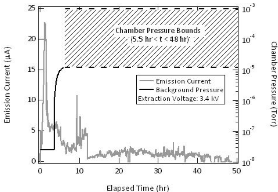
Figure 20. Electron emission current from the same quenched re-generable emitter used in the test of Figure 19. The emitter was held at a constant extraction voltage of 3.4 kV from t_e = 0.5 hr to t_e = 50 hr as background pressure was increased.
