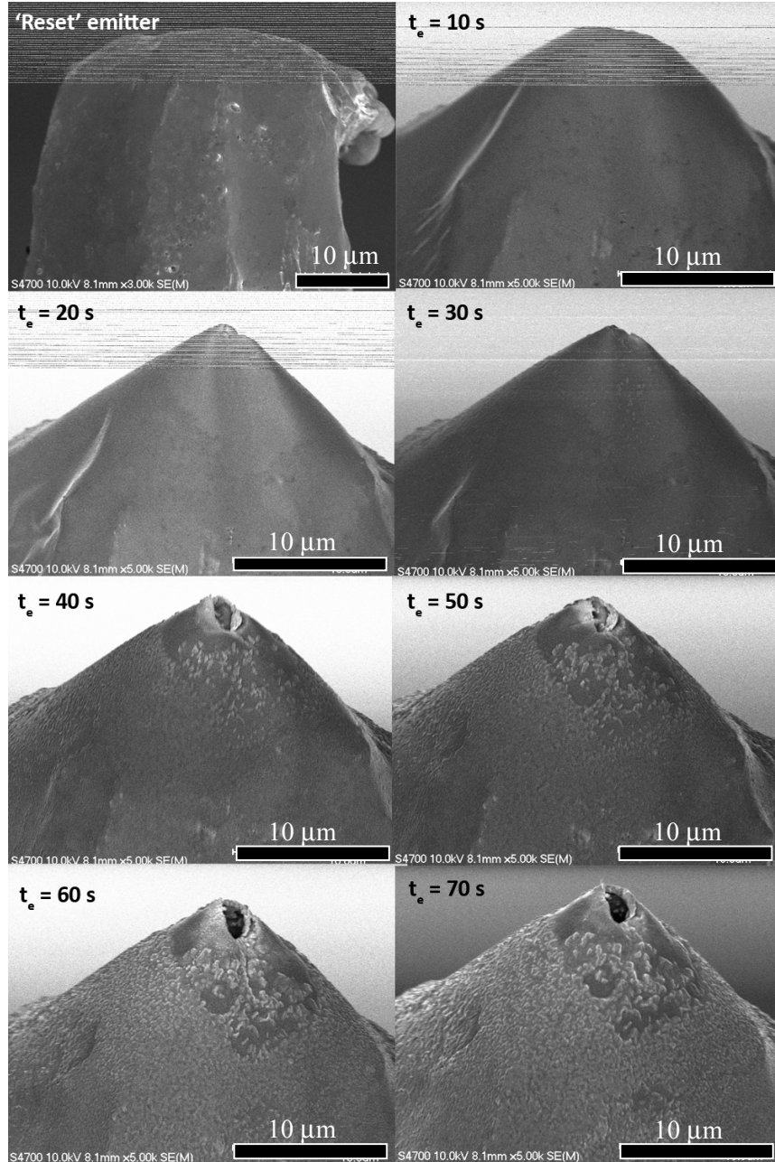
Figure 7. FE-SEM micrographs of the emitter tip taken after consecutive quenches at ion emission current of approximately 30 \mu A.
