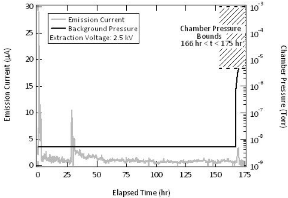
Figure 21. Extended duration experiment for an electron emitter that was re-generated by heating, acquiring ion emission, and then re-quenching after being damaged in the test sequences of Figure 19 to Figure 20. The extraction voltage was held constant at 2.5 kV from t_e = 1.5 hr to t_e = 175 hr and the test was ended by increasing the vacuum chamber pressure after over 150 hours of operation.
