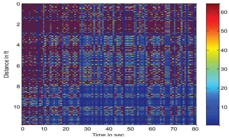
Figure 16 Eigen image of clutter for brick wall.
