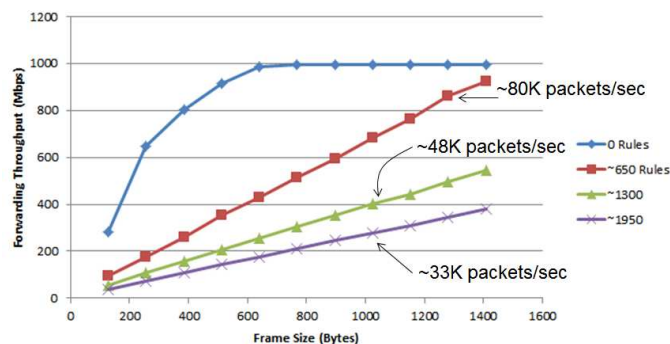
Figure 5. Proxy Throughput as Function of Filtering Rules
