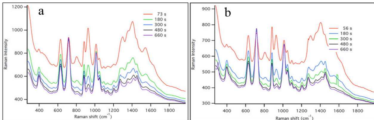
Figure 4. SERS spectra of 1.0 mM (a) and 5.0 mM (b) 2-mercaptoethanol obtained from planar substrates of tethered silver nanoparticles.
