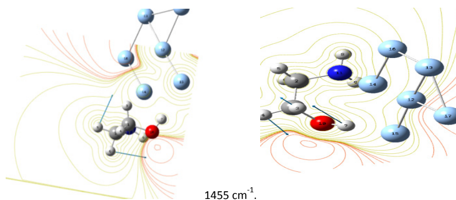
Figure 10. A weakly enhanced mode at 1455\text{ cm}^{-1} compared to a strongly enhanced mode at 1354\text{ cm}^{-1} for the aminoethanol + 6 Ag system. The atomic motions for the mode are indicated by vectors; the magnitude of the vectors is indicated by their length. A contour plot of the electrostatic potential is shown in the plane of the normal mode motion, where the electric field is directed normal to the equipotential lines and the magnitude of the field is indicated by the spacing of the equipotentials. For the mode that is strongly enhanced, atomic motions are mostly aligned with the electric field, and as indicated by the equipotential lines, the overall electric field is directed in one direction.
