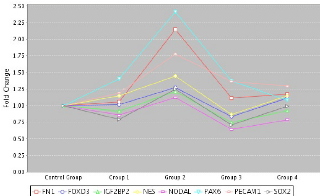
Figure 2. Genes up-regulated in cells exposed to 100 \mu M MP. PAX6 = Paired Box 6, a regulator of gene transcription in nervous/ocular system, FN1 = fibronectin 1, a glycoprotein involved in embryogenesis, PE-CAM1 = platelet/endothelial cell adhesion molecule, protein of IG superfamily, NES = Nestin, an inter-medicate filament protein in central nervous system (CNS) stem cells.
