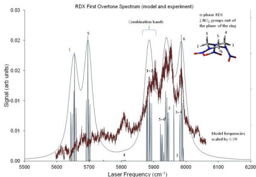
Figure 5. Comparison of the experimentally measured overtone and combination band vibrational spectra for RDX from eight positions in a cluster model.
