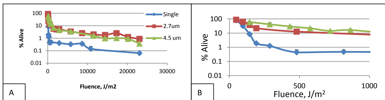
Figure 3. The UV-C kill curve for the single and clustered Bg (2.7 and 4.5 \mu\text{m} ) deposited on filter surfaces. (A) Kill curve for fluence up to 30,000 J/m 2 . (B) Kill curve for fluence up to 1,000 J/m 2 .
