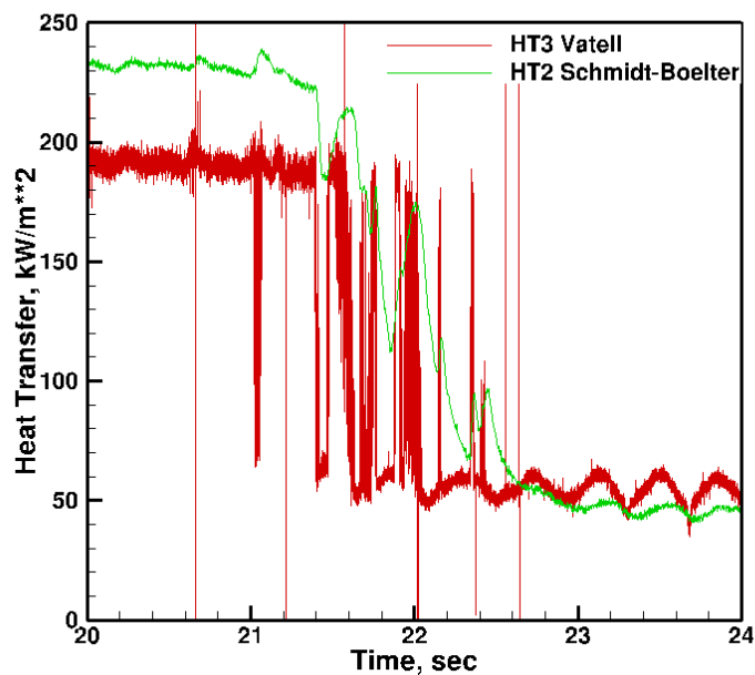
Figure 26 Comparison of Vatel heat transfer gauge and Medtherm Schmidt-Boelter heat transfer gauge.
