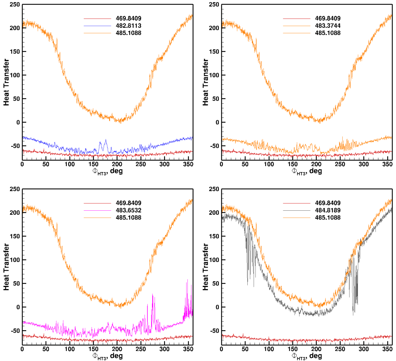
Figure 32 Vattel heat transfer guage HT3 signal during descent.
