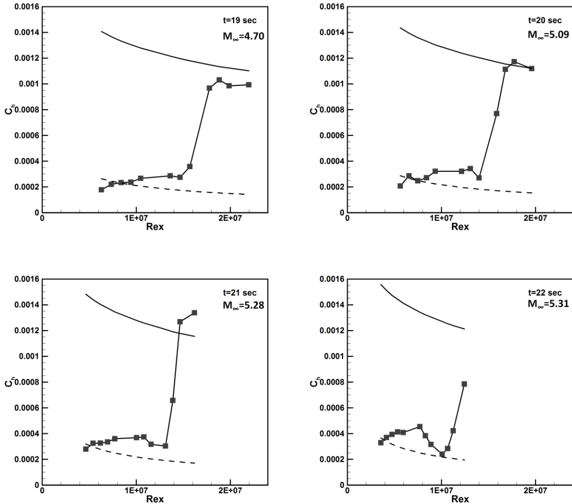
Figure 22 Heat transfer distributions. Symbols – flight data, dashed – Eckert, solid – van Driest.
