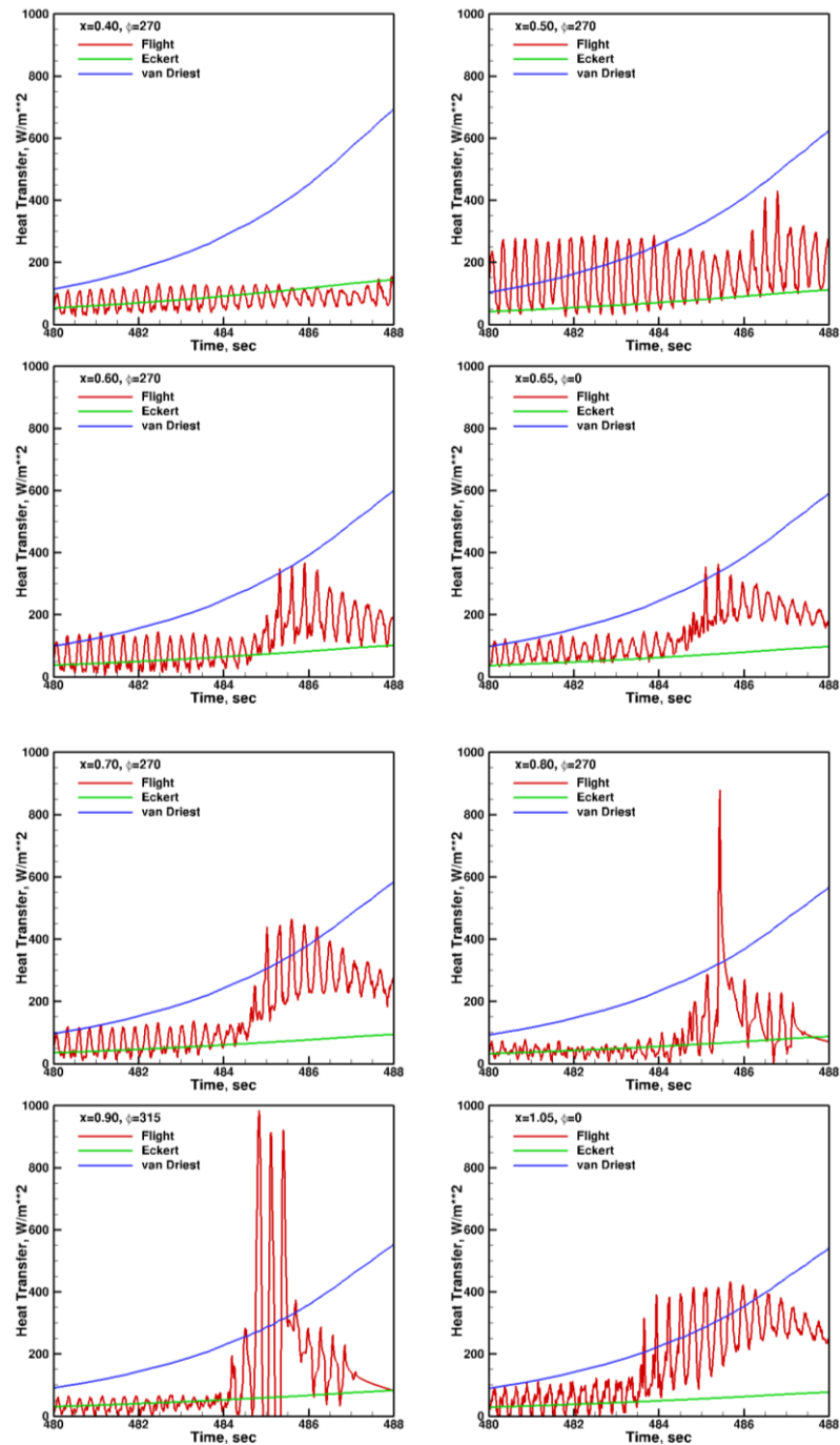
Figure 30 Reentry transition measured with Medtherm thermocouples.
