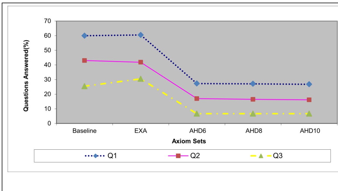
Figure 3.8: Effect of removal of high degree nodes on completeness
