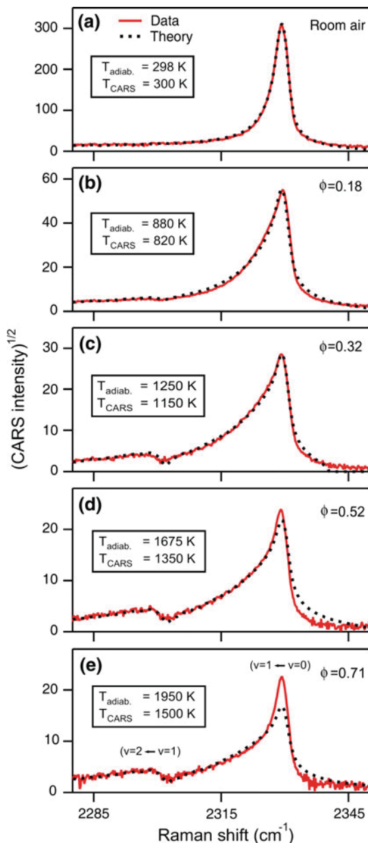
Fig. 10 Experimental (solid curves) and theoretical (dashed curves) fiber-based ps-CARS spectra of N_2 at a room temperature, b flame \phi = 0.18 , c flame \phi = 0.32 , d flame \phi = 0.52 , and e flame \phi = 0.71
