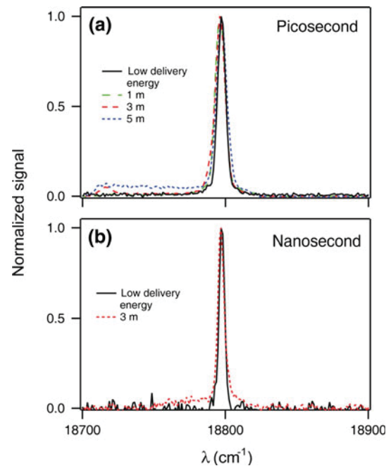
Fig. 5 a Measured power spectra for 150-ps laser-beam propagating through 1-m (dashed line, green), 3-m (dashed line, red), and 5-m-long (dashed line, blue) fiber at constant laser fluence ( 204\text{ mJ/cm}^2 ). Spectra for low laser fluence ( <1\text{ mJ/cm}^2 ) are same for each length and are shown as black solid line. b Measured power spectra for 8-ns laser beam propagating through a 3-m-long fiber at high fluence of 1,020\text{ mJ/cm}^2 (dashed line, red) and low fluence of <1\text{ mJ/cm}^2 (solid line, black)
