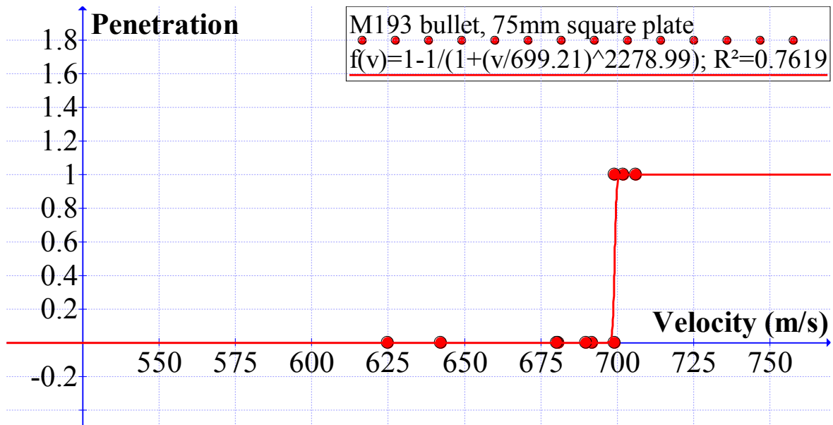
Figure 5: Penetration of M193 bullet in 75mm square steel plate. Regression analysis shows V_{50}=699.21 m/s.
