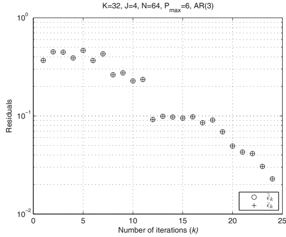
Fig. 7. Residuals \bar{\epsilon}_{Jp} and \hat{\epsilon}_{Jp} for model order selection in CG-PAMF ( K = 32 ; J = 4 ; N = 64 ; P = 3 ; \bar{P} = 6 )
