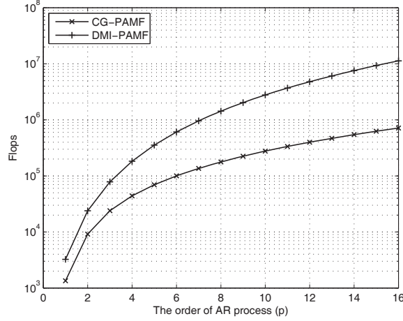
Fig. 12. Computational complexity of CG-PAMF and DMI-PAMF versus AR model order p ( K = 32 ; J = 8 ; N = 32 ).
