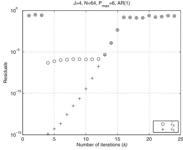
Fig. 4. Residuals \bar{\epsilon}_{JP} and \hat{\epsilon}_{JP} for model order selection in CG-PMF ( J = 4 ; N = 64 ; P = 1 ; \bar{P} = 6 )
