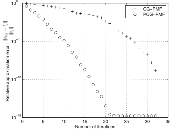
Fig. 8. Convergence of CG-PMF and PCG-PMF ( J = 4 ; P = 8 )
