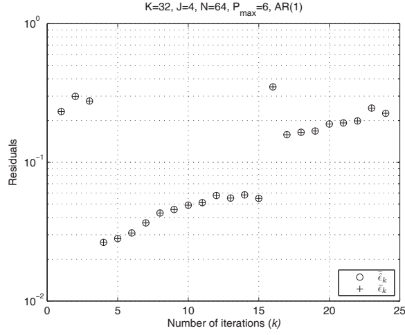
Fig. 6. Residuals \bar{\epsilon}_{Jp} and \hat{\epsilon}_{Jp} for model order selection in CG-PAMF ( K = 32 ; J = 4 ; N = 64 ; P = 1 ; \bar{P} = 6 )
