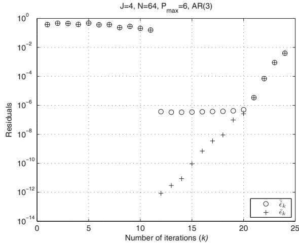
Fig. 5. Residuals \bar{\epsilon}_{JP} and \hat{\epsilon}_{JP} for model order selection in CG-PMF ( J = 4 ; N = 64 ; P = 3 ; \bar{P} = 6 )
