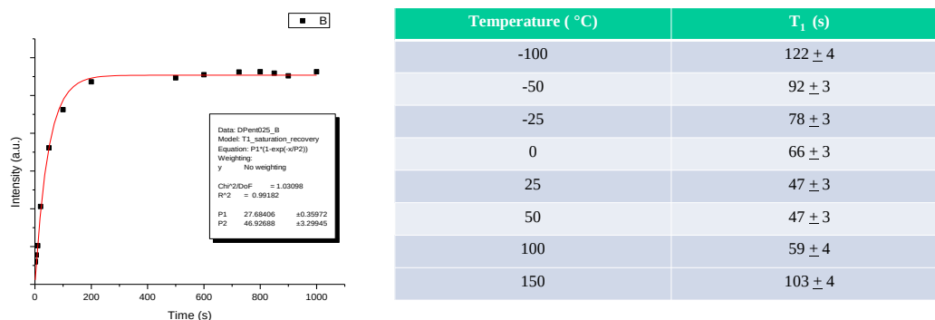
Figure 6. Relaxation Data for Lightly Doped Pentacene Sample (0.17mol% spins).
