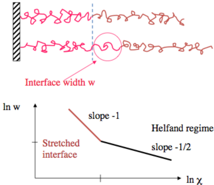
Figure 1. Relationship of the interfacial width relative to c for block copolymer brushes
