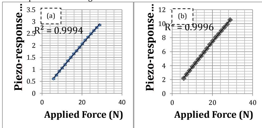
Fig 8: Piezo-response of: (a) AlN thin film deposited at 5mtorr of working pressure, 1kW of power, 1.0 microsecond of reverse time and 20% of nitrogen/argon ratio. (b) AlN thin film deposited at 5mtorr of working pressure, 1kW of power, 1.0 microsecond of reverse time and 80% of nitrogen/argon ratio.
