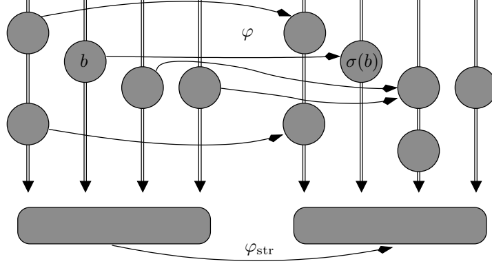
Figure 7: Protomorphism of Protoskeletons
