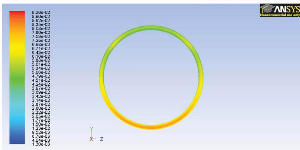
Figure 5.17: Contours of density at isolator outlet for angles of attack of 0^\circ , 3^\circ and 6^\circ .
