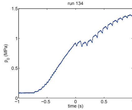
Figure 5: Sample barrel pressure history, result for run 134 shown.
