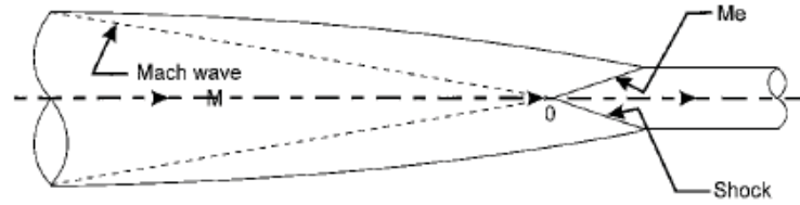
Figure 2.15: Generating flow field for modular stream traced inlet design (Billig & Kothari, 2000).
