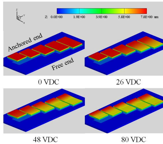
Figure 32. Cantilever actuation simulated with CoventorWare ® to determine the biasing voltage necessary to draw the cantilevers to the actuation pads.
