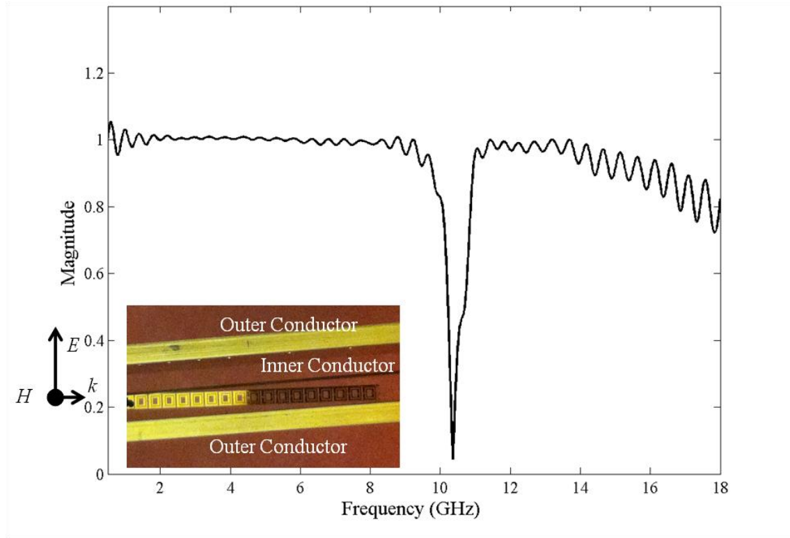
Figure 46. The transmission magnitude response captured for the 10 – 15 GHz Baseline meta-atom showing the resonant frequency occurring just above 10 GHz. The inset shows a 10 – 15 GHz Baseline meta-atom inserted in the RF strip-line between the inner and outer conductor.
