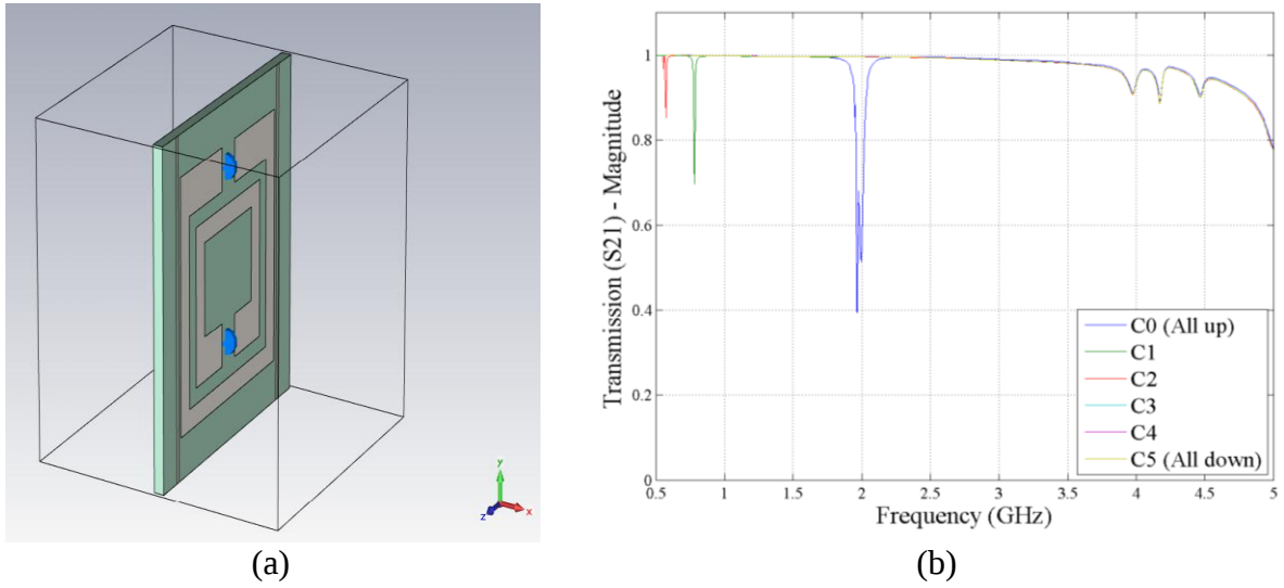
Figure 40. 1 – 4 GHz meta-atom integrated with cantilevers. The cantilevers are simulated with lumped elements capacitors.
