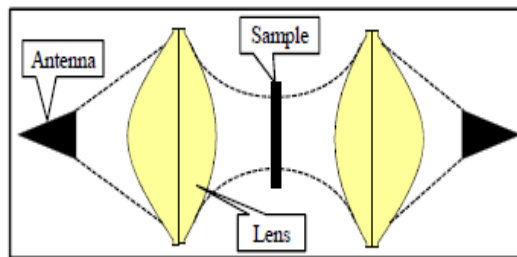
Figure 60. Schematic of a focused beam system [71].
