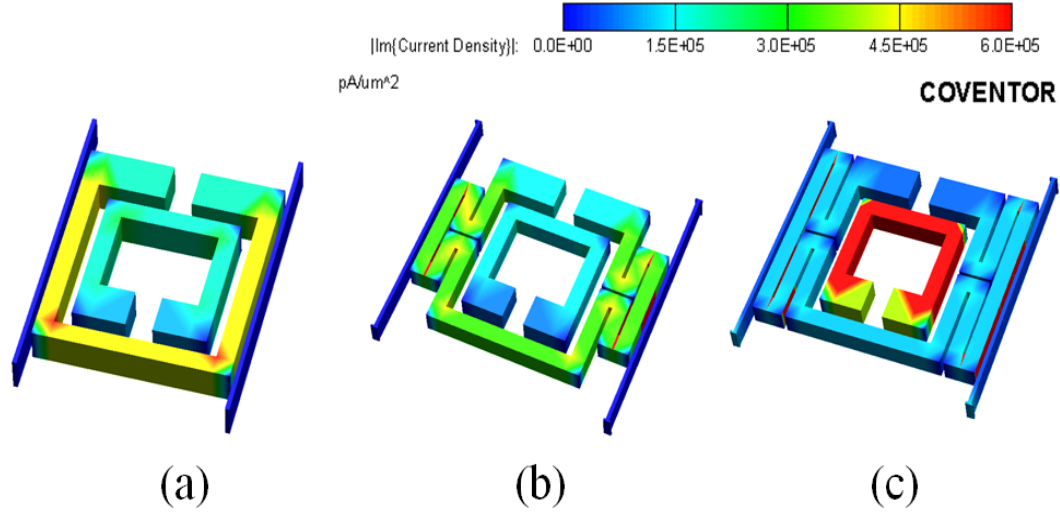
Figure 37. CoventorWare® plots showing magnitude of imaginary current density incident on the (a) Baseline, (b) Loop A and (c) Loop B versions of the meta-atom designs. Changes in the imaginary current density were observed as the length of each loop increased from the Baseline to the Loop B design. The magnitude of the imaginary current density increases on the inner split ring resonator which is relative to the increase in inductance and capacitance. However, the magnitude of the imaginary current density decreases for the outer split ring resonator.
