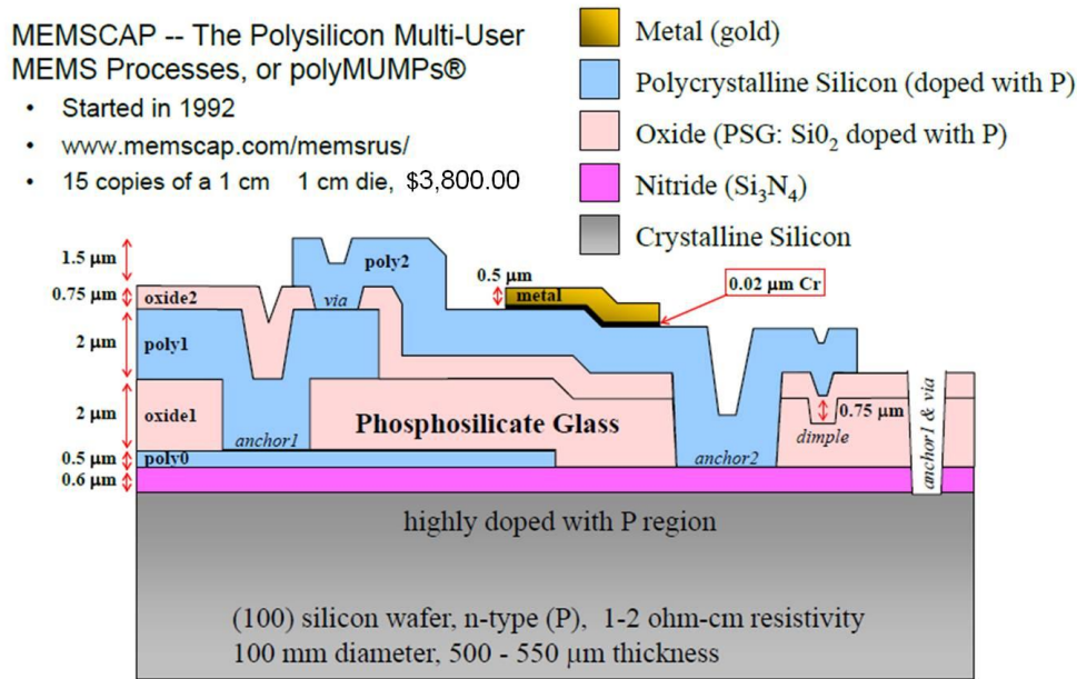
Figure 11. PolyMUMPS® layers and dimensions for MEMS. The layers provide structures to build devices with a surface micromachine process.
