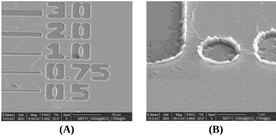
Figure 72 Metamaterial etching results
