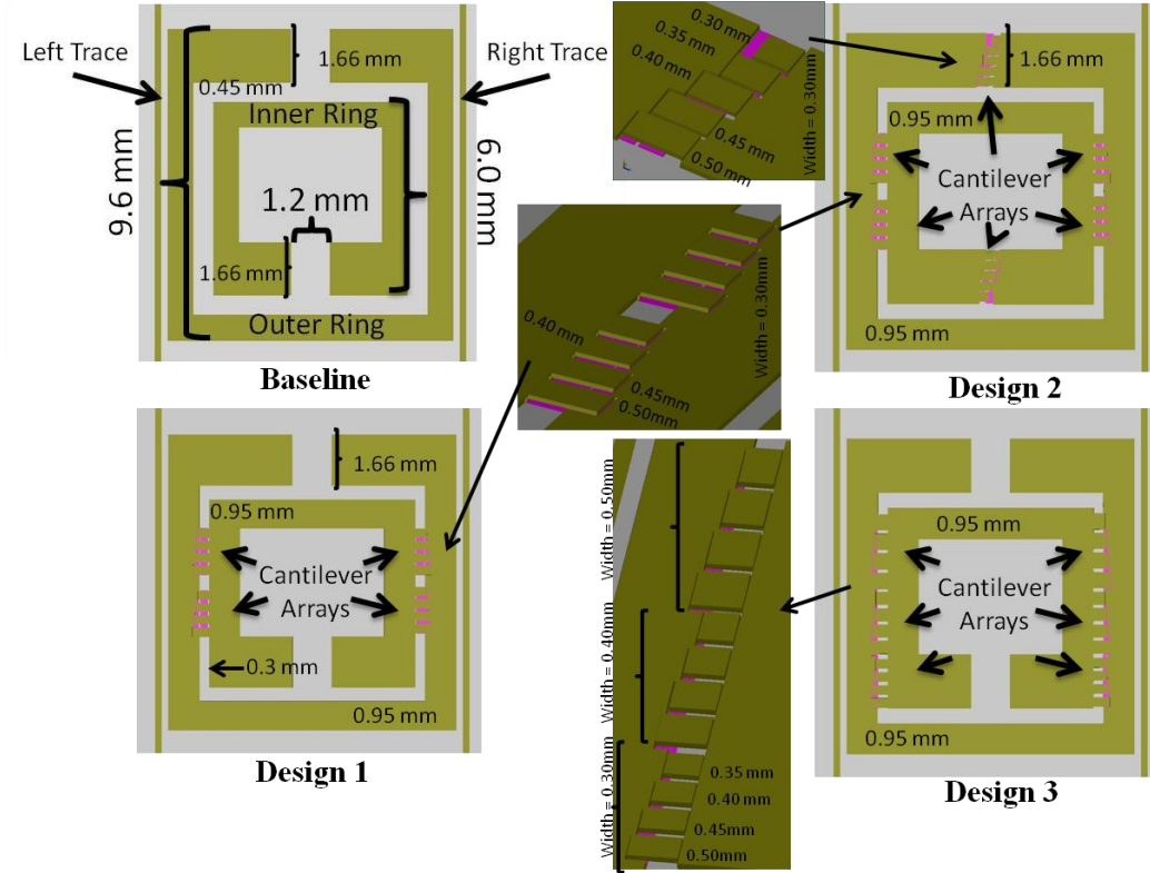
Figure 23. Layout of the three intra-ring meta-atom design variations integrated with (Design 1) cantilevers between rings, (Design 2) cantilevers in the gap and connecting the rings, and (Design 3) cantilevers with varying widths between the rings.
