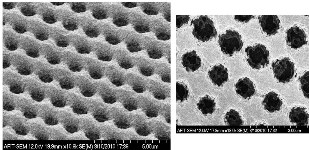
Figure 76. Interferometric Samples generated at Air Force Research Laboratory.
