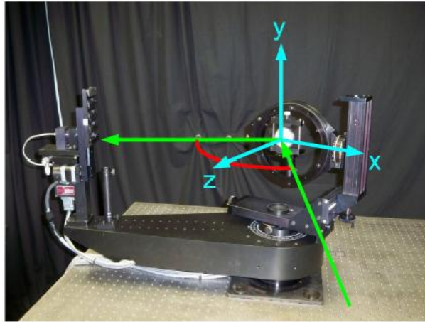
Figure 77. AFIT's complete angle scatter instrument used to measure bi-directional reflection distribution function for optical metamaterials.
