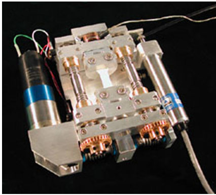
Figure 2. Ernest Fullam in-situ tension-compression stage
