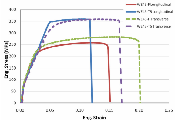
Figure 6. Example stress – strain curves of the -F and -T5 samples in the longitudinal and transverse directions.
