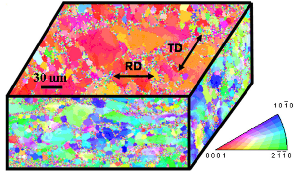
Figure 8. Schematic of the orientation texture of WE43-T5 in relation to the plate directions (not to scale).
