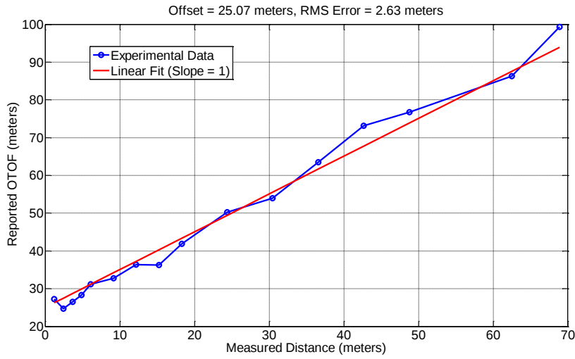
Figure 1. Correlation of measured and reported OTOF data for the outdoor case
