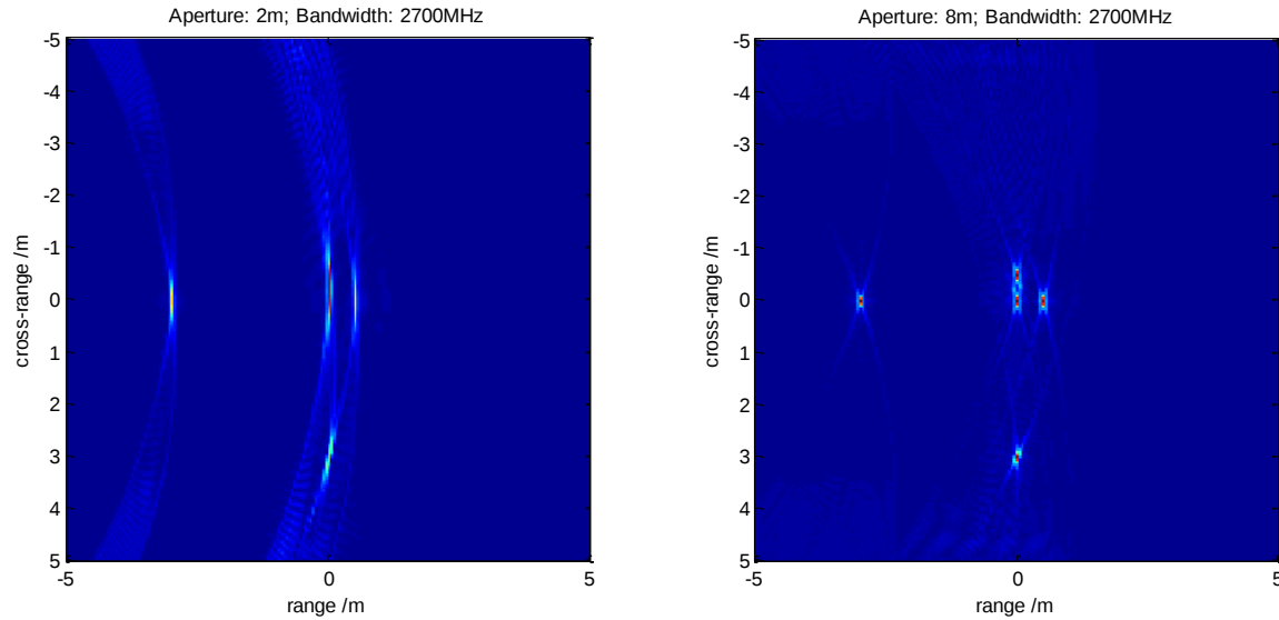
Figure 26 Simulated UWB SAR image with (left) regular aperture and (right) extended aperture.
