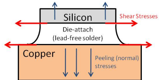
Figure 5: Bi-metal assembly representation of power MOSFET under thermo-mechanical loading.
