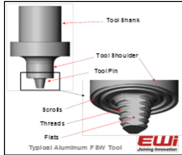
Figure 1. FSW tool.
