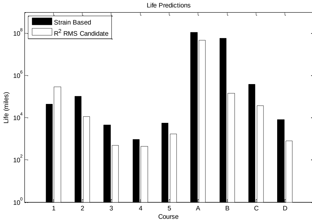
Figure 3: Life Estimate Using Coefficient of Determination of Root Mean Square
