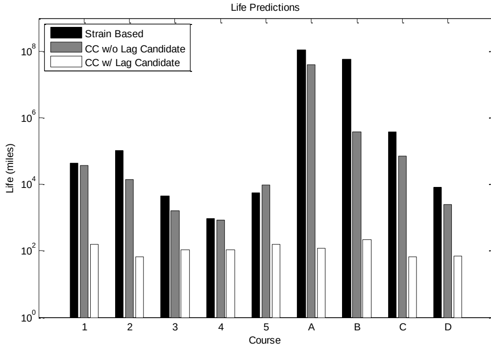
Figure 2: Life Estimate Using Cross-Correlation (CC)
