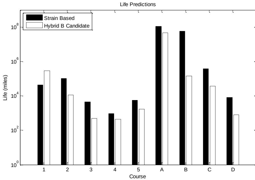
Figure 4: Life Estimate Using Hybrid B Model
