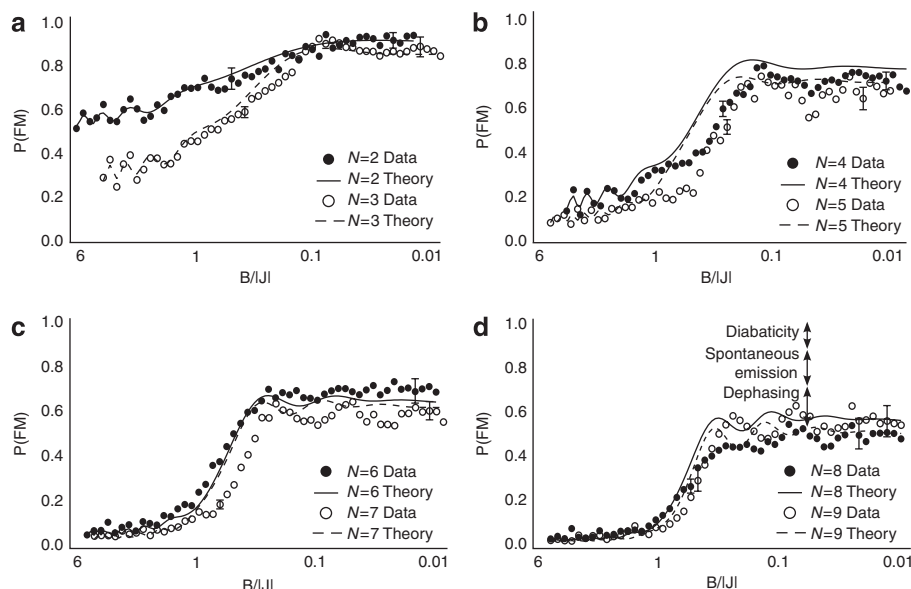
Figure 4 | Suppression of P(\text{FM}) with increasing number of spins. (a–d) Ferromagnetic order P(\text{FM}) = P(0) + P(N) is plotted vs B/|J| for N = 2 to N = 9 spins. The circles are experimental data, and the lines are theoretical results including decoherence and imperfect initialization. As this quantity includes only two of 2^N basis states, random spin-flips and other errors degrade it much faster than the magnetization and Binder cumulant. The representative detection error bars are shown on a few points for each N . The P(\text{FM}) reduces from \sim 0.9 to \sim 0.55 as the system size is increased from two to nine. The principle contribution to this degradation is decoherence, predominantly due to spontaneous emission from intermediate ^2P_{1/2} states in the Raman transition and additional dephasing, primarily due to intensity fluctuations in Raman beams. Shown in d is an estimated breakdown of the suppression of P(\text{FM}) from various effects for N = 9 spins. Non-adiabaticity due to finite ramping speed, and spontaneous emission and additional dephasing due to fluctuating Raman beams suppress P(\text{FM}) by \sim 8\% , \sim 18\% and \sim 24\% respectively from unity ( B/|J| \rightarrow 0 ).
