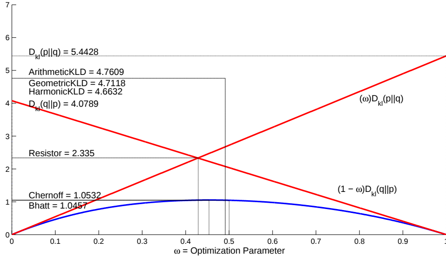
Figure 3.10: Relationships between various information divergences [134]
