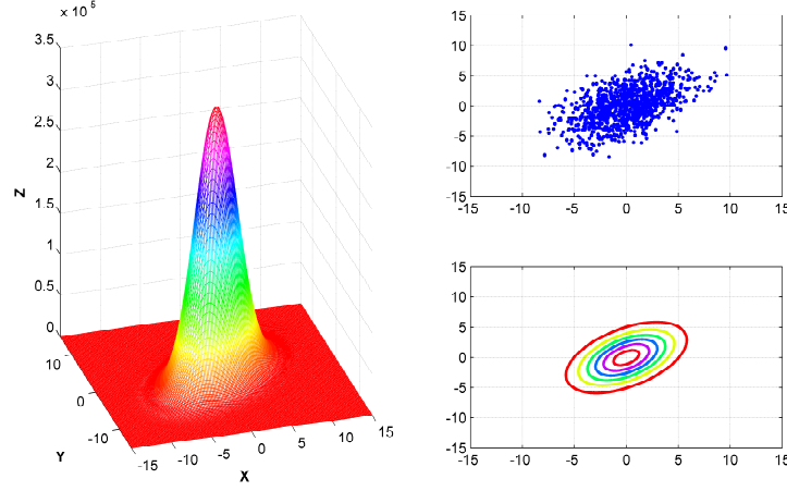
Figure 2.12: Gaussian probability density function, 1000 monte carlo samples, and associated contour plot.
