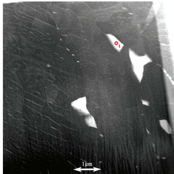
Figure 18. TEM image of bulk microstructure, the large precipitate that was indexed is marked.
