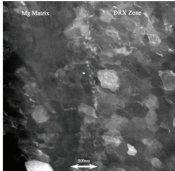
Figure 17. TEM image of transition zone interfacing the DRX region and neighboring microstructure.
