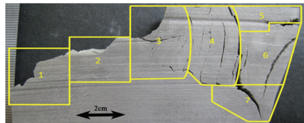
Figure 13. Map of sectioned samples of C-Partial
