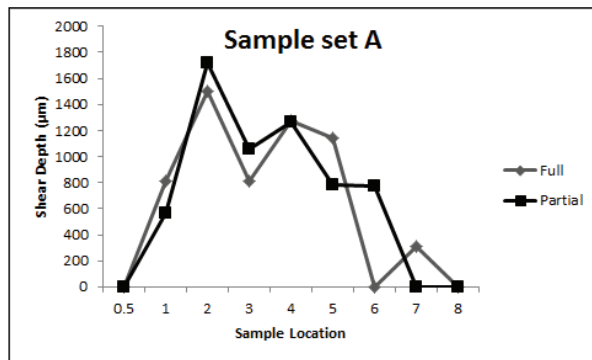
Figure 10. Shear localization depth of sample set A.
