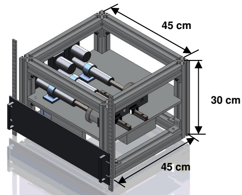
Figure 1. FLEA test stand engineering model
