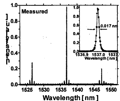
Measured Vernier expansion of FSR in cascaded pair of resonators.
