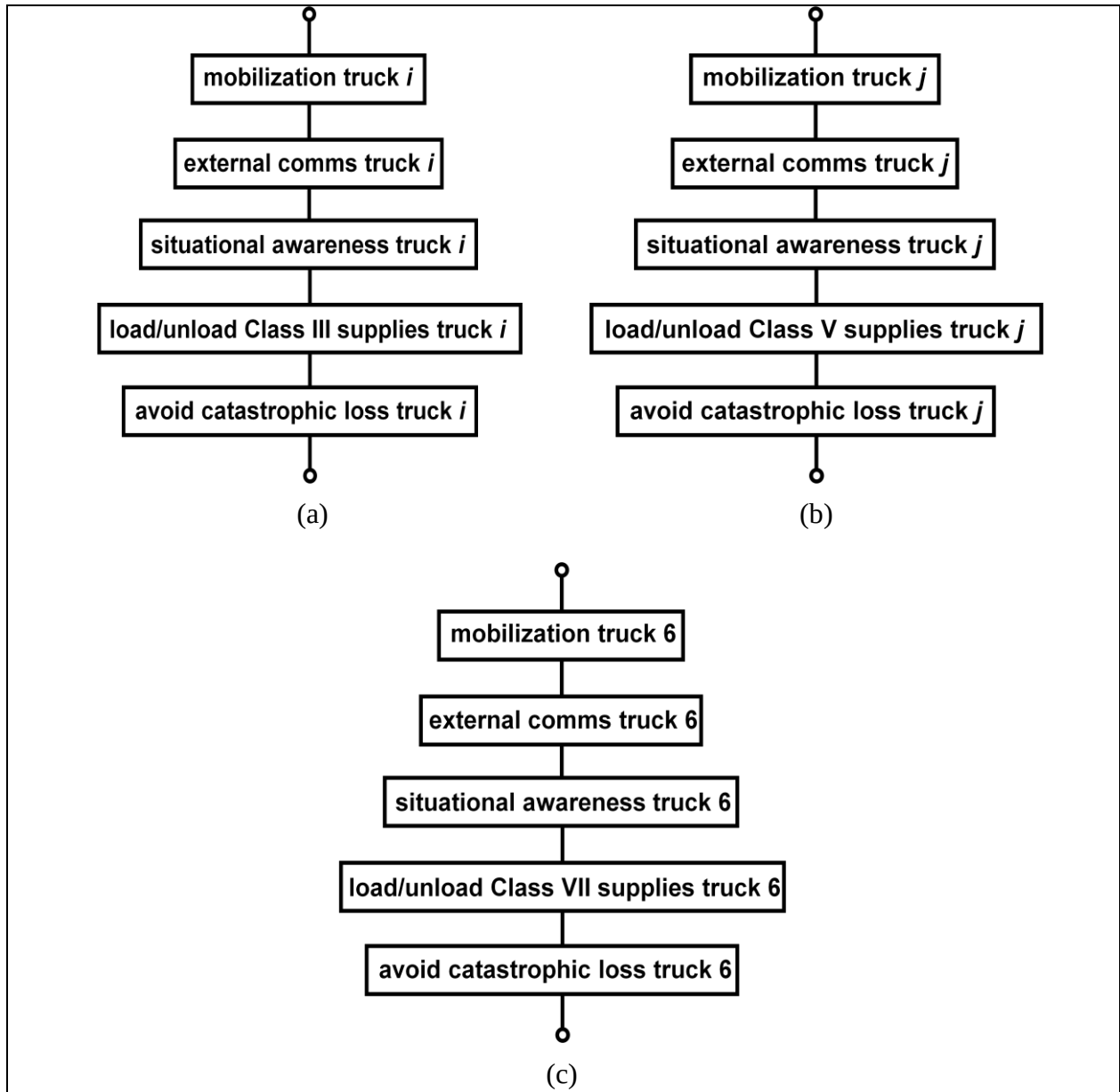
Figure A-7. Fault tree diagrams illustrating the generalized “provide supplies” task readiness states associated with (a) the i^{\text{th}} truck providing class III supplies, (b) the j^{\text{th}} truck providing class V supplies, and (c) truck 6 providing class VII supplies.
