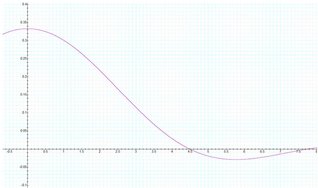
Figure F.1: The graph of the function f in (F.9).
