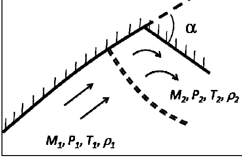
Figure 6. Oblique shock wave with deflection angle \alpha near the bending corner of the damaged area is shown by the dashed bended lines. Parameters of the incident and aftershock flows are indicated by sub-indexes 1 and 2 respectively.
