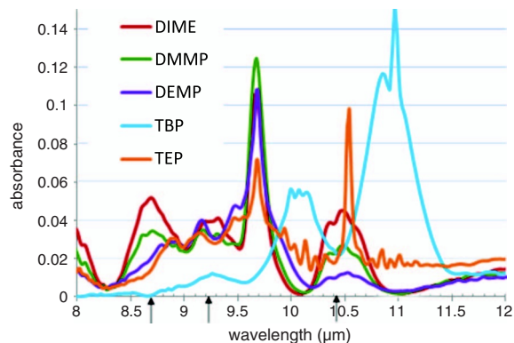
Fig. 2. Representative measured absorbance spectra for the five nerve agent simulants, where the arrows identify the three laser wavelengths at 8.68, 9.29, and 10.35 \mu\text{m} .
