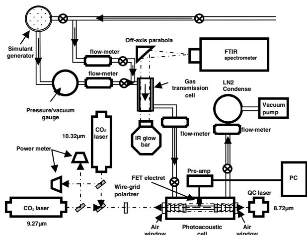
Fig. 1. Schematic of the multiwavelength LPAS experiment.
