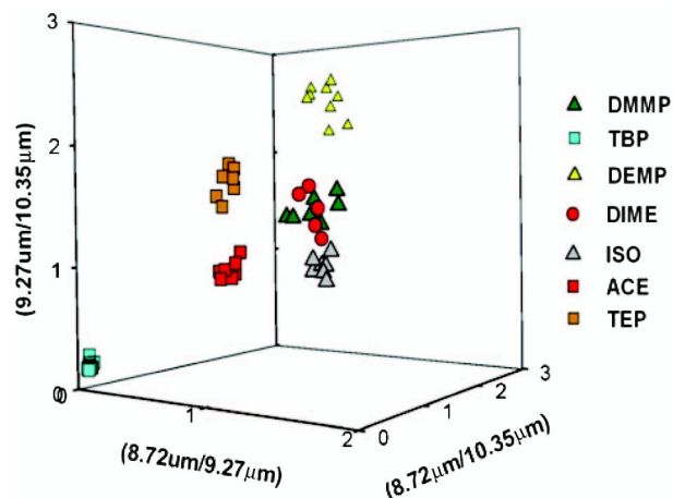
Fig. 3. Ratios of the absorption response for the three wavelengths are shown for the five nerve agent simulants and two volatile organic compounds.
