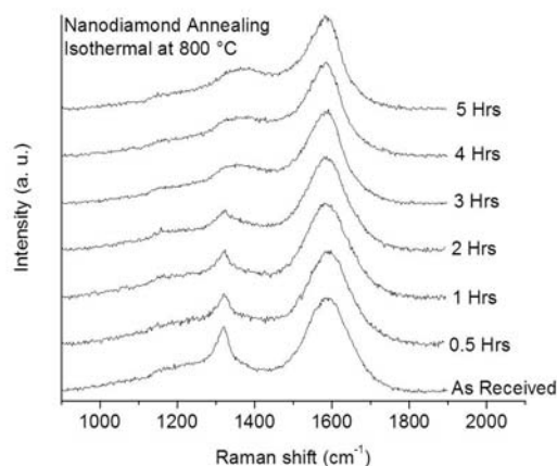
Figure 25. Changes in Raman spectra of ND powder after annealing at 800 °C for 0.5, 1, 2, 3, 4, and 5 hrs.
