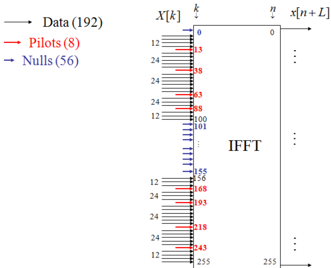
Figure 4. Mapping of the IFFT inputs to time-domain outputs for 802.16 for N=256 subcarriers. From [3].
