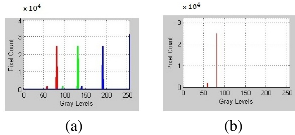
Figure 3.10: Threshold Extraction: Determine a threshold for each color, e.g., by use of color histograms: (a) histogram for all three color bands, (b) histogram associated only with the red band.
