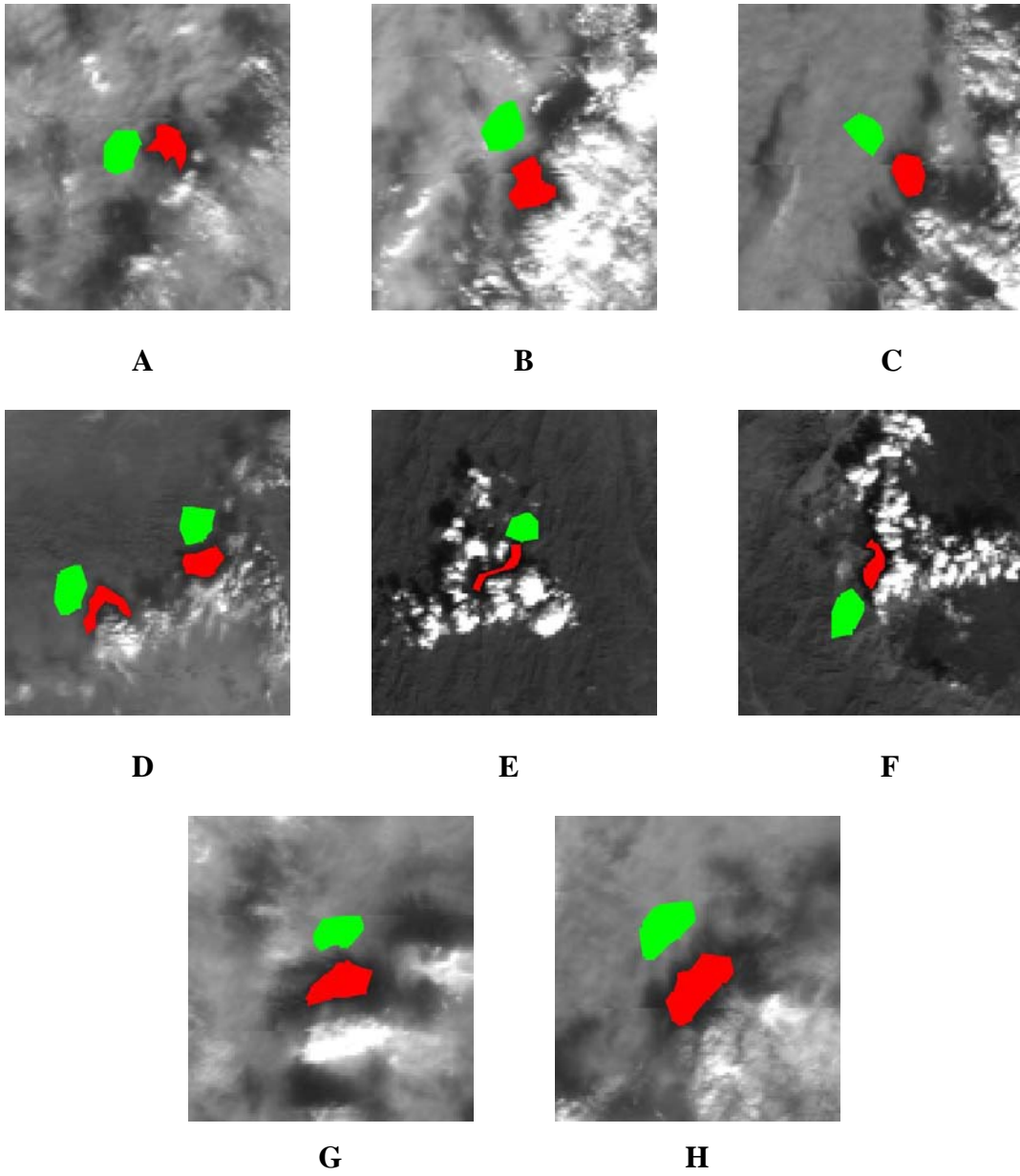
Figure 11. Cloud Pairs from Iran and Afghanistan, December 11, 2003. A) Pair 1. B) Pair 2. C) Pair 3. D): Pair 4 (left) and Pair 5. E) Pair 6. F) Pair 7. G) Pair 8. H) Pair 9.
