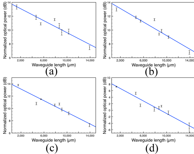
Fig. 4. (a), (b) The transmitted optical power as a function of waveguide length is shown for two different sets of measurements of the best chip, with losses of 4.3 \pm 0.6 dB/cm and 4.9 \pm 0.6 dB/cm achieved. (c), (d) The
